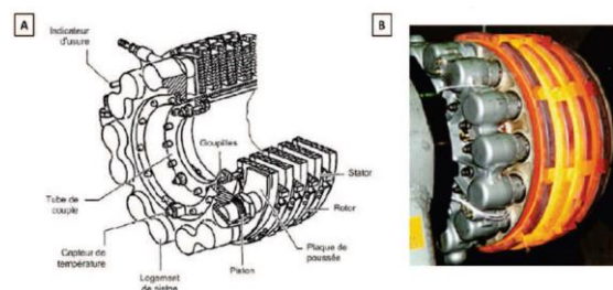
Fig 1: Principle of a heat well (Raud 2018)
